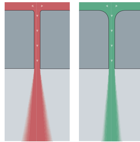
Non-original nozzle element without after treatment Spray angle = 15.3° Droplet size = 14.4 µm
