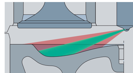
Non-original nozzle element without after treatment
