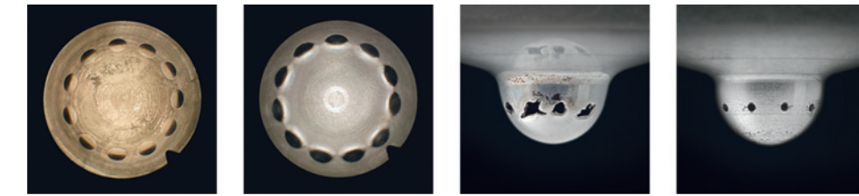
The non-original injector nozzle fuel delivery ports without after treatment could lead to fuel nozzle cracks, injector tip failure and consequential damages to the injector sleeve.
